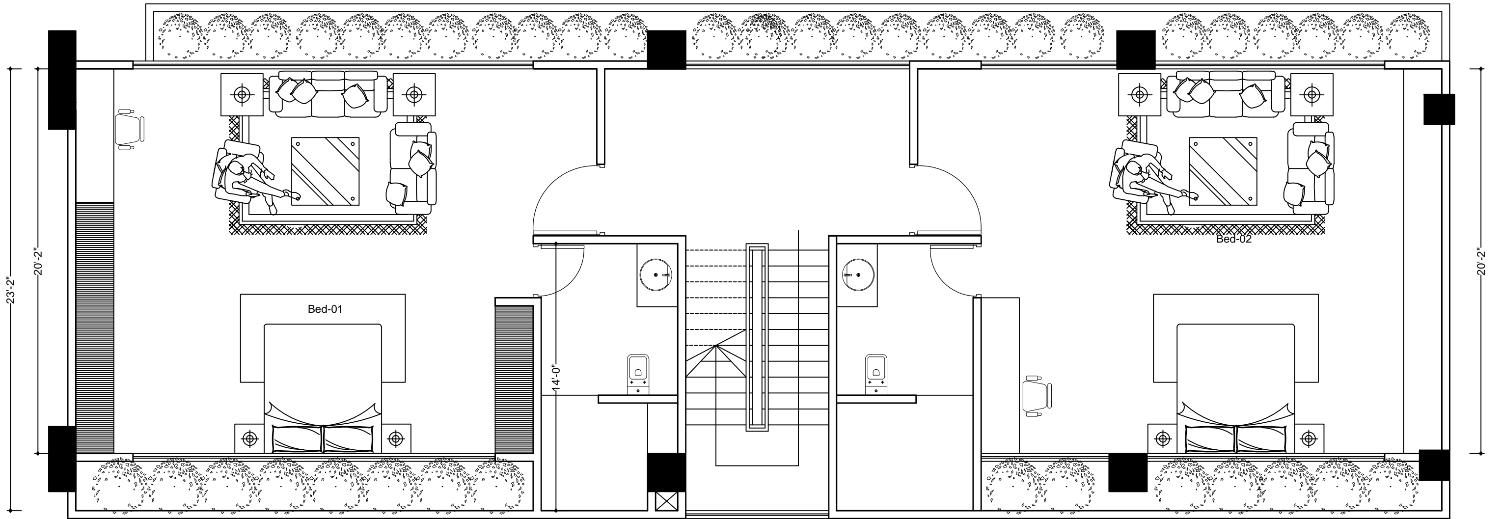
8th Floor Plan 1740 sft
