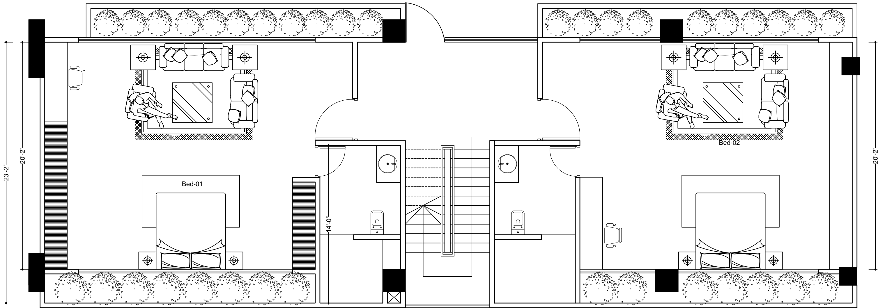
7th Floor Plan 1740 sft
